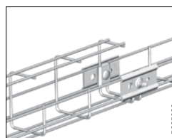
Fittings B1 and B2 are used for joining the mesh trays. Example of joining G-mesh tray with standard mesh tray
