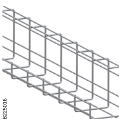
G-Mesh tray 120x150
