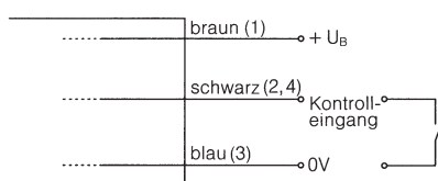
③ Sender
